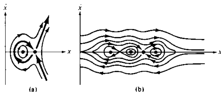
Figure 12 Phase curves
