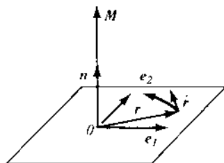
Figure 28 Angular momentum
