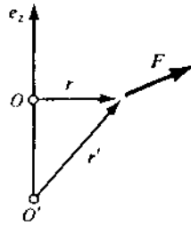
Figure 37 Moment of the vector F with respect to an axis
