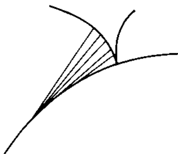
Figure 252 An evolute of a curve
