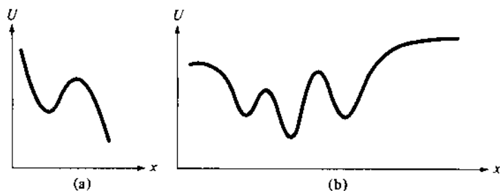
Figure 11 Potential energy
