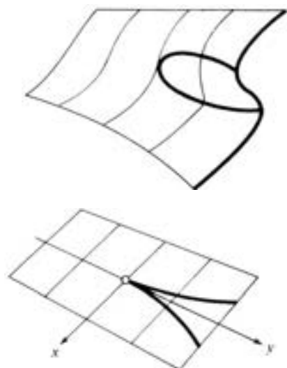
Figure 245 Whitney's tuck
