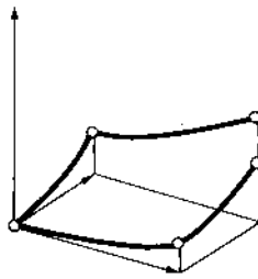
Figure 236 Integral curves constructed for a non-integrable field of planes
