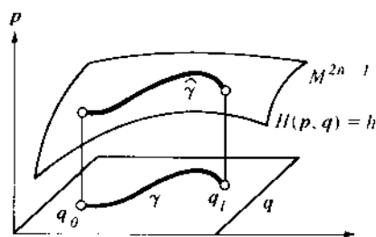
Figure 189 Maupertuis' principle
