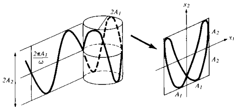
Figure 19 Construction of a Lissajous figure
