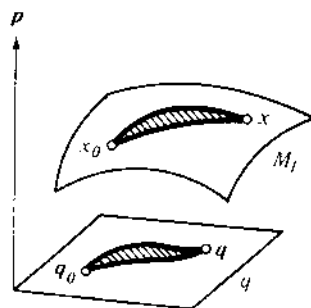
Figure 219 Independence of the path for the integral of \mathbf{p} dq on M_f
