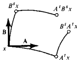
Figure 169 Non-commutative flows
