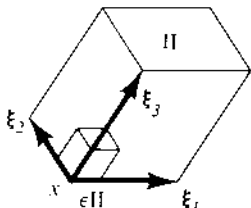
Figure 155 Definition of divergence of a vector field
