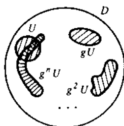
Figure 51 Theorem on returning
