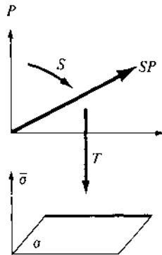
Figure 209 Checking non-degeneracy
