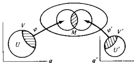
Figure 56 Compatible charts
