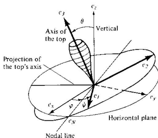
Figure 126 Euler angles
