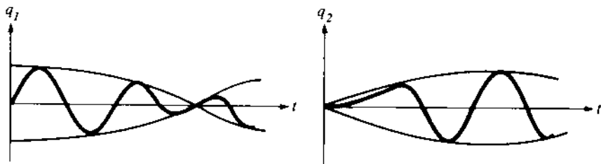
Figure 83 Beats
