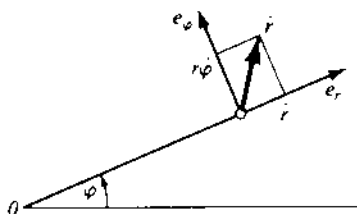
Figure 29 Decomposition of the vector \dot{r} in terms of the basis e_r, e_\phi
