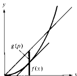
Figure 46 Legendre transformation of a quadratic form
