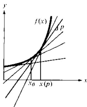
Figure 45 Involutivity of the Legendre transformation
