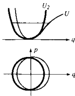
Figure 76 Linearization
