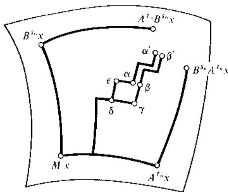
Figure 171 Curvilinear quadrilateral \beta; \delta \epsilon \alpha
