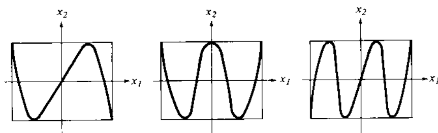
Figure 24 Chebyshev polynomials
