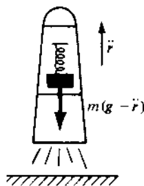
Figure 107 Overload
