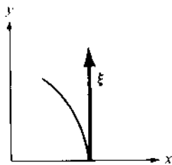
Figure 141 Problem 1
