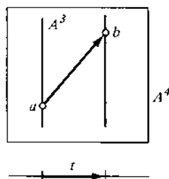
Figure 2 Interval of time t
